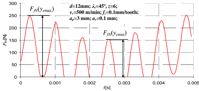
Fig. 2. The experimental time course of F_{fN} normal feed force component with the designation of instantaneous force corresponding to maximum F_{fN}(y_{e\max}) and minimum F_{fN}(y_{e\min}) cutter displacement envelope.
