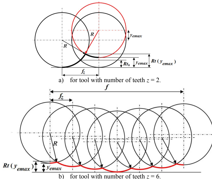
Fig. 1. Projection of the cutter into the work piece including cutter displacement, where: R – tool radius, f – feed per revolution, f_z – feed per tooth, y_{max} – maximum value of cutter displacement envelope, Rt(y_{max}) – surface roughness height including cutter displacement, Rt_0 – theoretical surface roughness.
