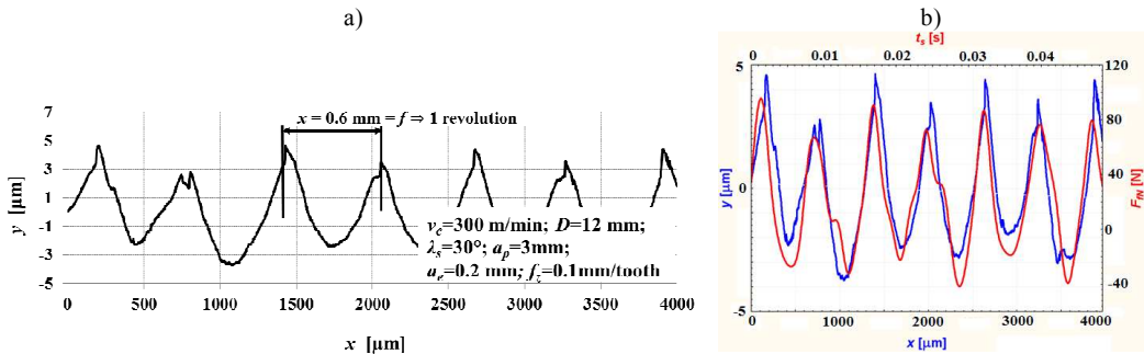
Fig. 6. a) surface profile chart; b) surface profile chart (blue line) with superimposed envelope of F_{FN} force (red line) for v_c = 300 m/min.
