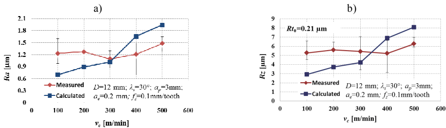
Fig. 9. a) surface roughness Ra in function of cutting speed v_c ; b) surface roughness Rz in function of cutting speed v_c .
