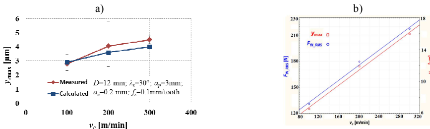
Fig. 8. a) maximum instantaneous displacement envelope y_{emax} per tool revolution in function of cutting speed v_c ; b) maximum instantaneous total displacement y_{max} per each tooth and feed normal force F_{FN\_RMS} in function of cutting speed v_c .
