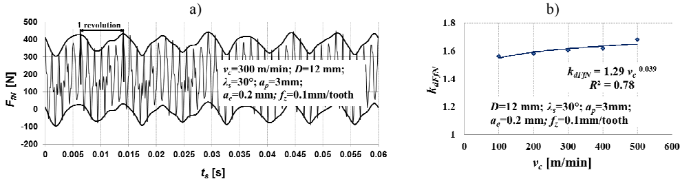
Fig. 5. a) time course for feed normal force component F_{FN} (thick black line denotes the envelope of F_{FN} force); b) dynamics coefficient k_{dF_{FN}} in function of cutting speed v_c .
