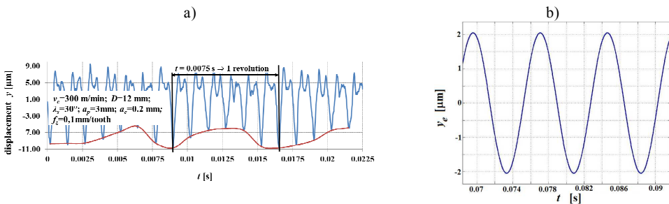
Fig. 7. a) the time course of measured total cutter displacement y (red line denotes the envelope of displacement y_e ) for v_c = 300 m/min; b) the time course of simulated envelope of cutter displacement y_e for v_c = 300 m/min.
