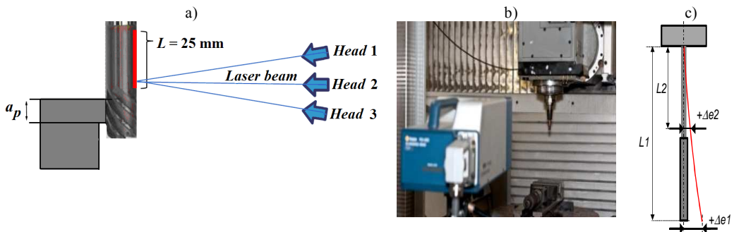
Fig. 4. Tool displacement measurement diagram: a) block scheme of 3D displacement measurement carried out on a scanning vibrometer; b) the view of laser head (no. 1) during the calibration process; c) the scheme of cutter displacement.
