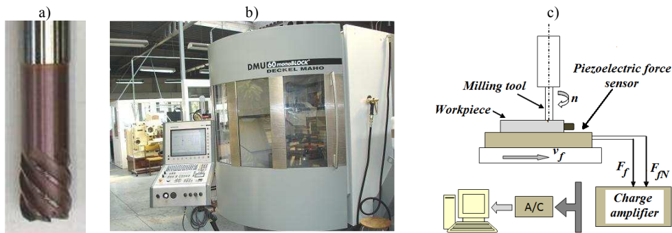
Fig. 3. Milling process experimental stand: a) the view of the employed tool; b) the view of DMG model DMU 60monoBLOCK milling center; c) block scheme of cutting force experimental apparatus.
